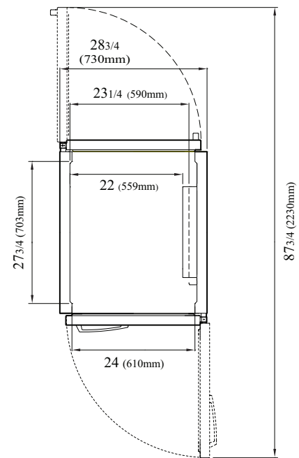
TOP VIEW
